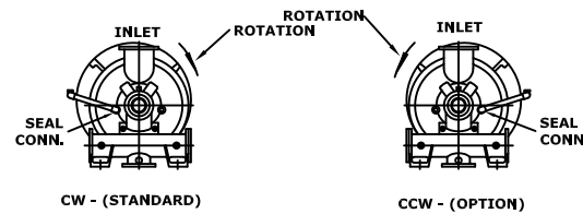
ASSY POSITIONS (FACING DRIVE END)
