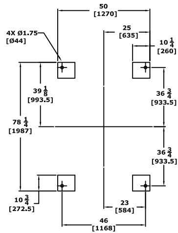
PUMP FOOTING
