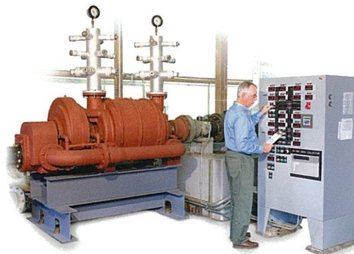
A Vooner FloGard high-vacuum two-stage pump VTS-20 being tested in Charlotte, NC.
